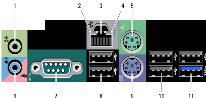
Figur 2. Oversigt over bagpanel
