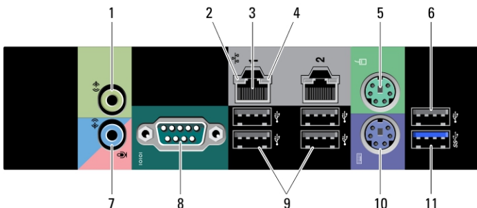
Figur 4. Oversigt over bagpanel
